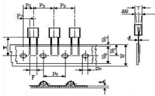
Fig.1 P=5.0, 7.5mm
