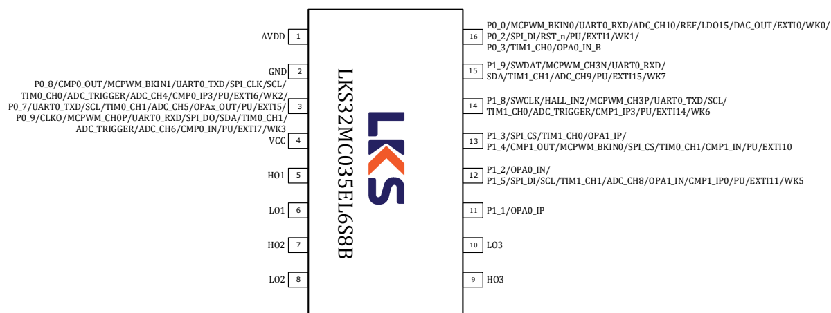
Figure 3-7 LKS32MC035EL6S8B(C) Pin Assignment Diagram
