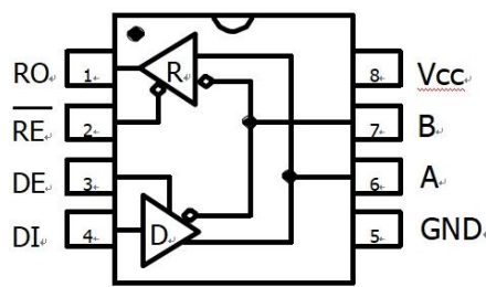
DIP-8/SOP-8/MSOP-8
