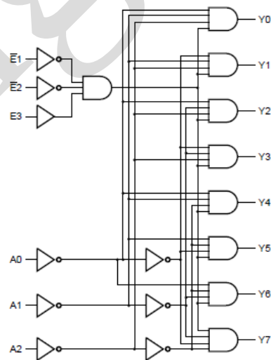
Figure 3. Logic diagram
