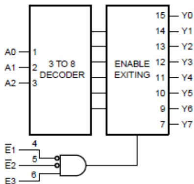
Figure 1. Logic symbol
