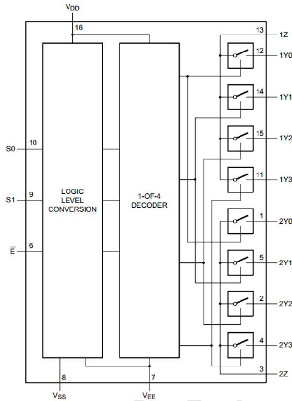
Figure 4. Functional diagram
