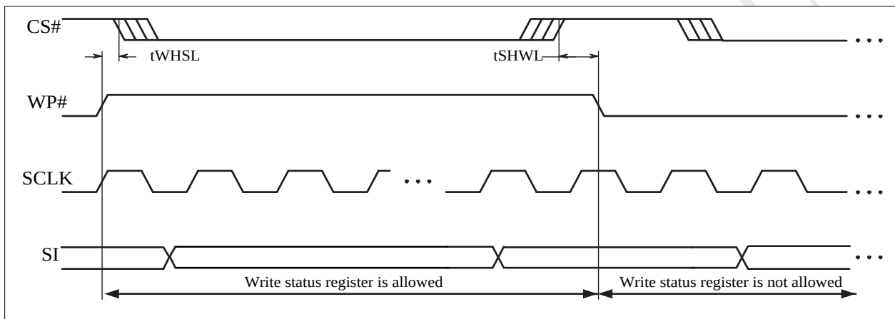
Figure 5-7 WP Timing
