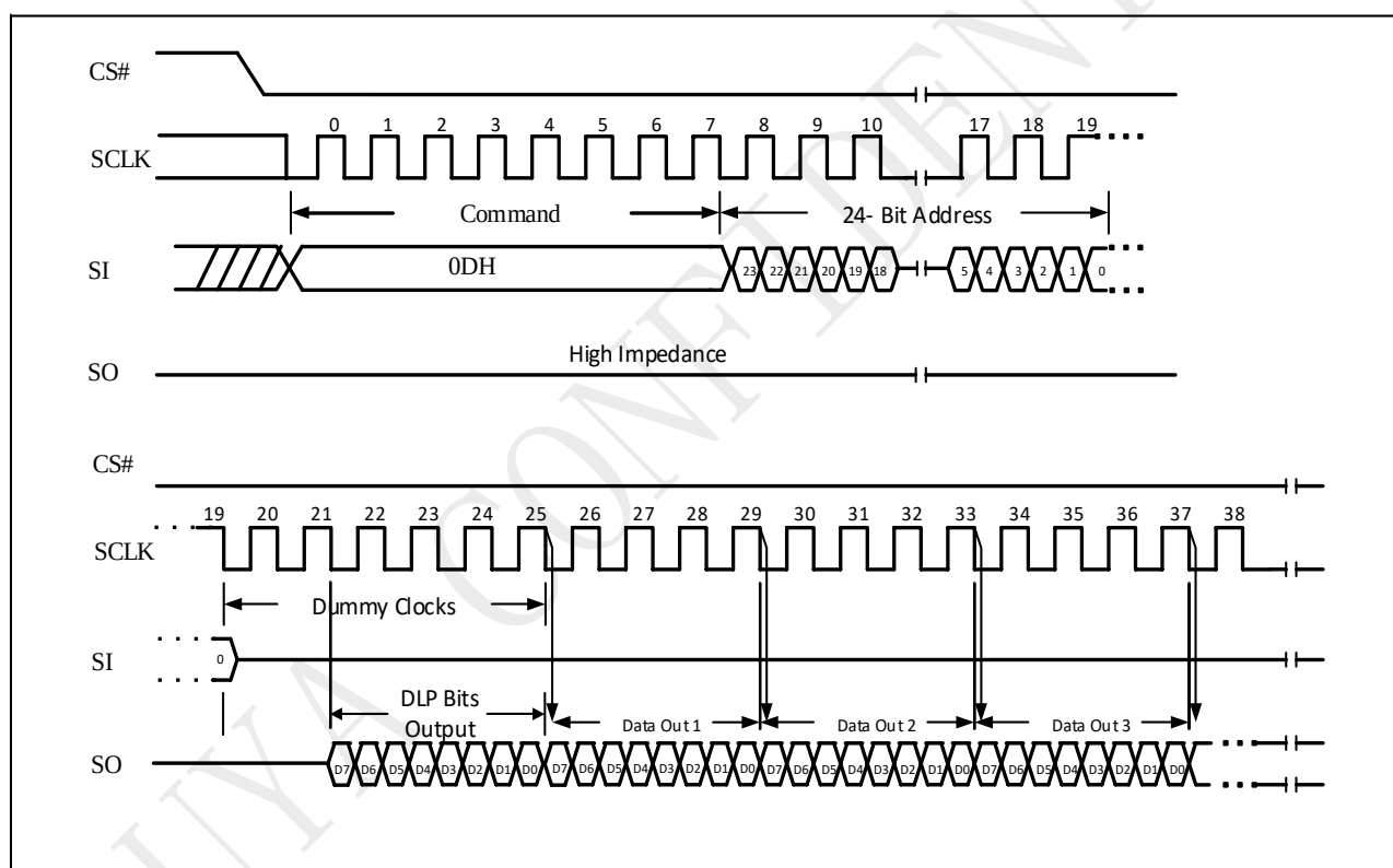
Figure 10-23i DTR Fast Read with DLP bits output Sequence
