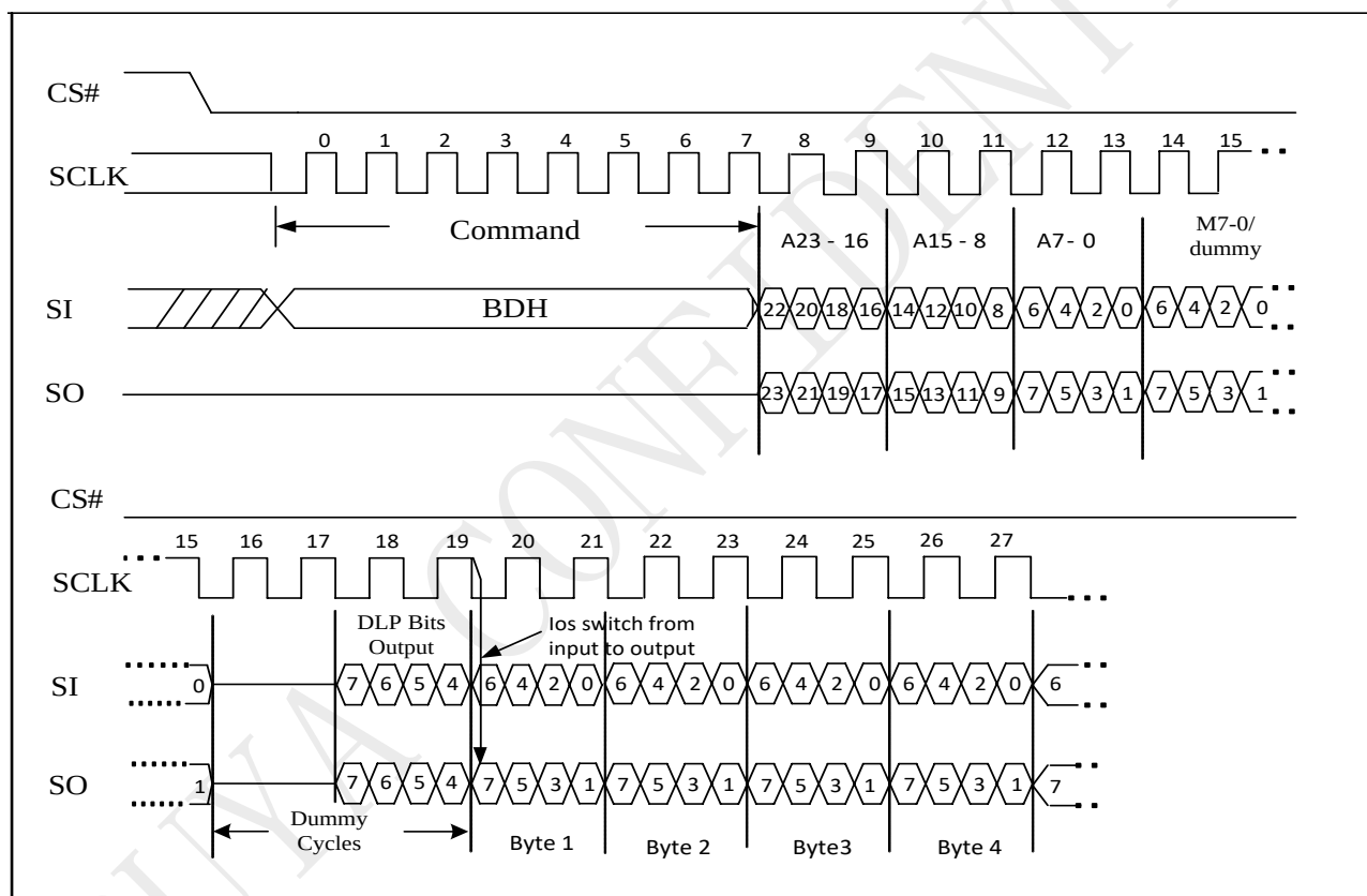
Figure 10-23k DTR 2IO Read with DLP bits output Sequence
