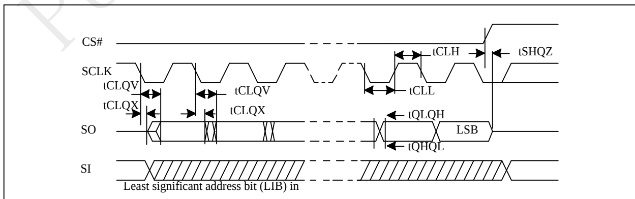
Figure 5-5 Output Timing
