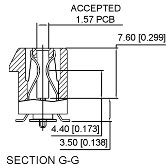
SECTION G-G
