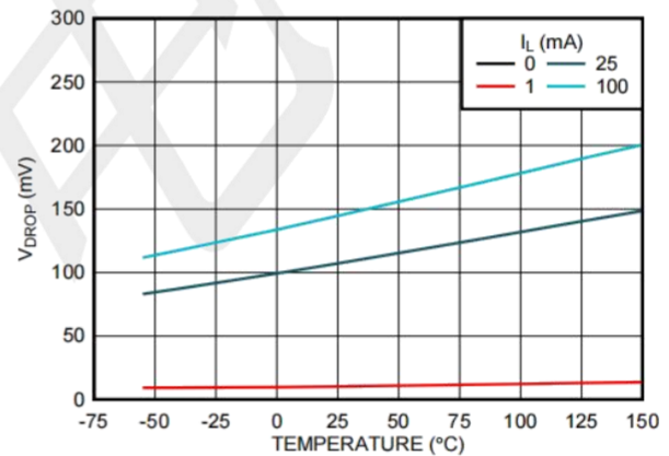
Dropout Voltage ( V_{DRO} ) versus Temperature
