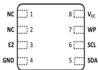
DFN-8 2*3
