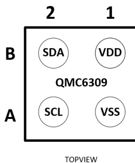
Figure 3. Package Top View
