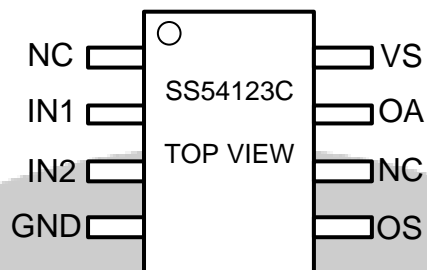
Figure 4. Pin Configuration
