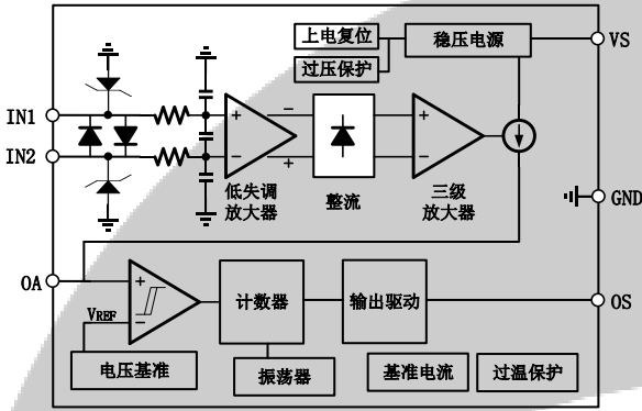
Figure 5. SS54123C Block Diagram
