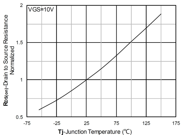
Normalized On-Resistance
