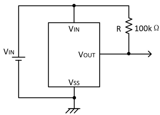
N-ch Open Drain Output
