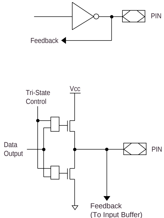
Typical Output
