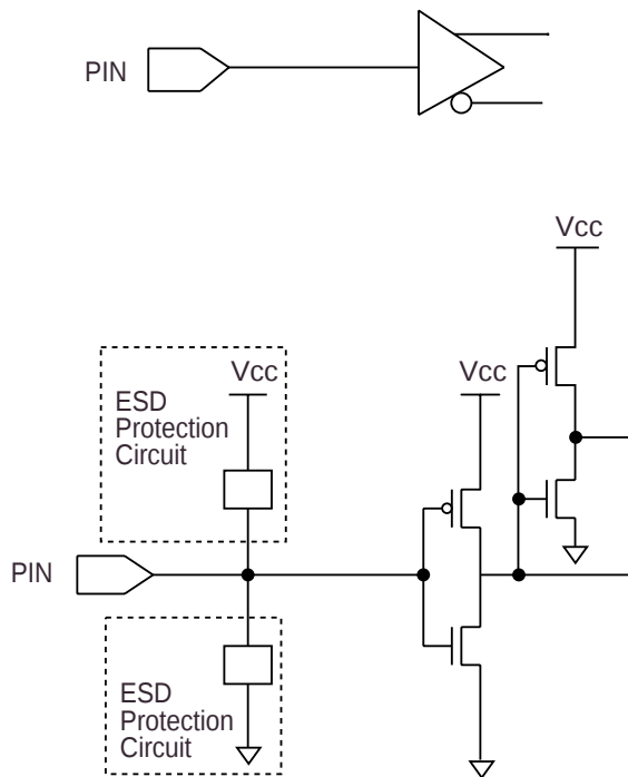
Typical Input
