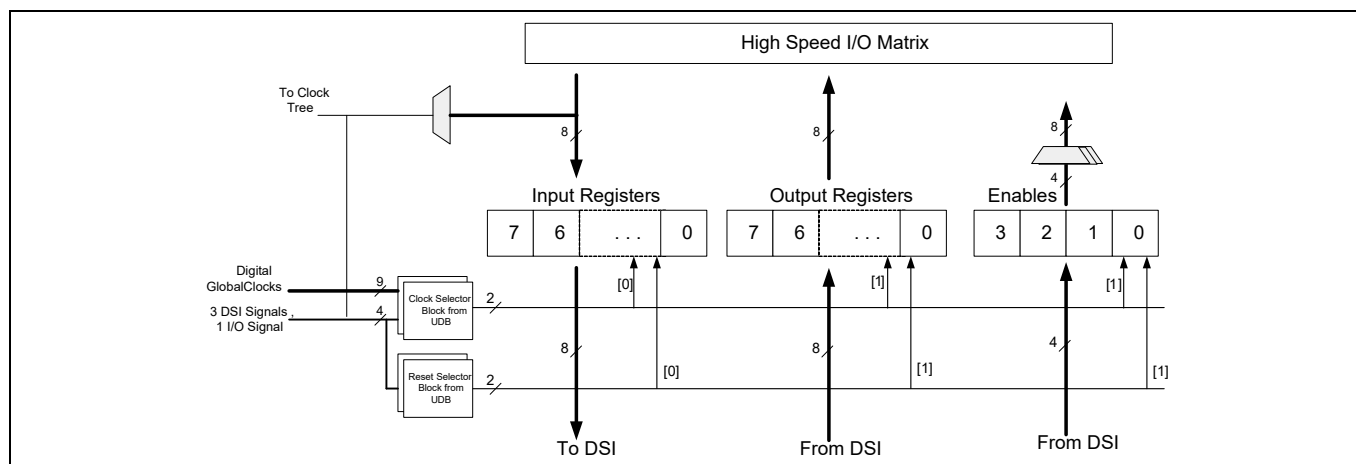
Figure 7 Port Interface
