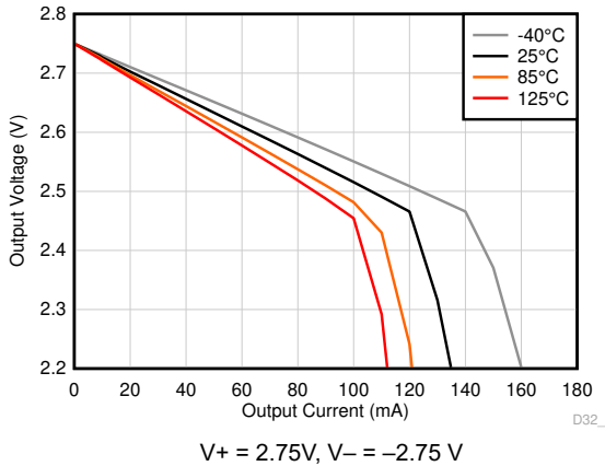
Figure 6-21. Output Voltage Swing vs Output Current (Sourcing)
