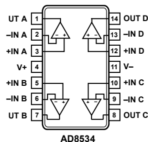
Figure 4. 14-Lead SOP and 14-Lead TSSOP (R and RU Suffixes)
