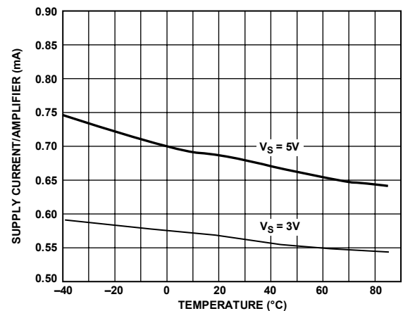
Figure 29. Supply Current per Amplifier vs. Temperature
