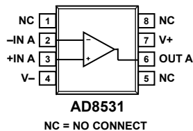
Figure 2. 8-Lead SOP (R Suffix)
