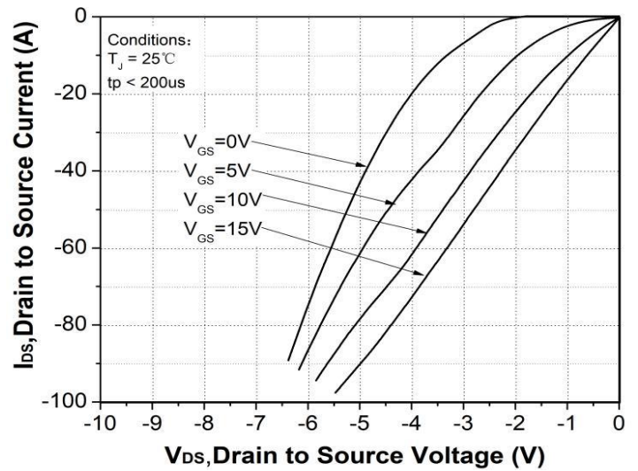
Figure 14. 3rd quadrant characteristic at T_J = 25\text{ }^\circ\text{C}
