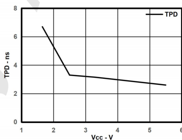
Fig. 8-2. TPD Across V_{CC} at 25^\circ\text{C}
