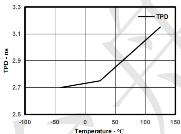
Fig. 8-1. TPD Across Temperature AT 3.3 V V_{CC}
