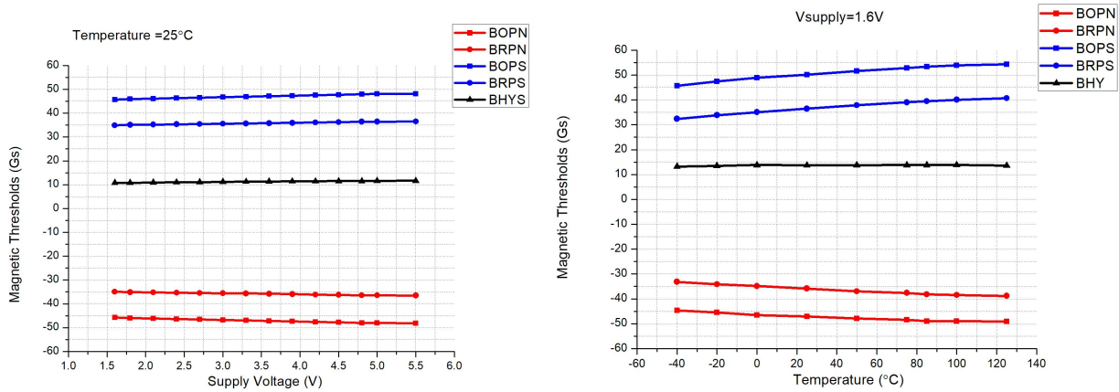
磁场阈值 vs. 供电电压 @T A =25°C
