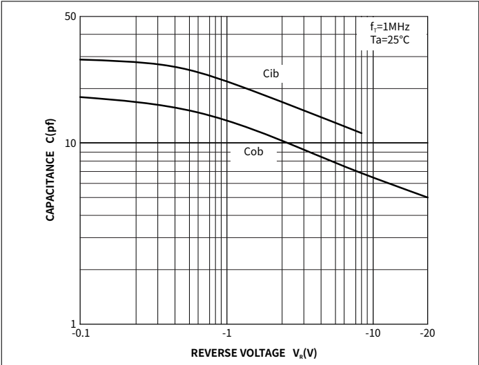
Fig.6 Cob/Cib- V_{be}
