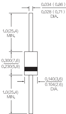
DO-204AC(DO-15)
