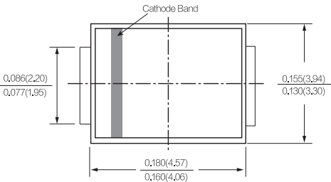
DO-214AA (SMB)
