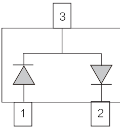
BAT54S
