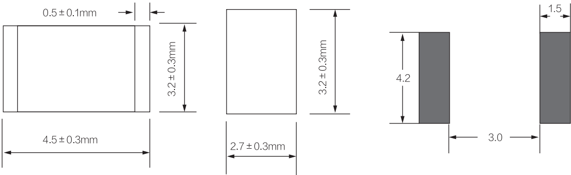
Mounting Pad Layout
