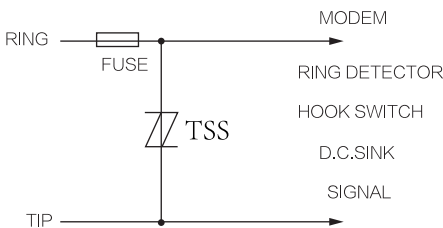
Modem Inter-wire Protection
