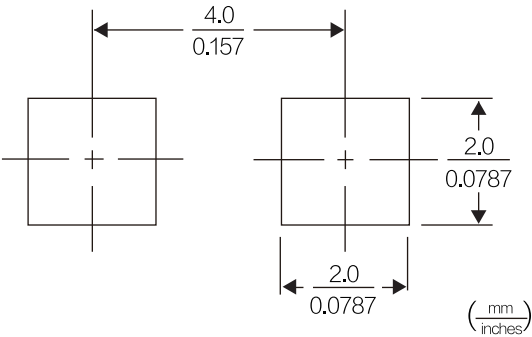
PCB Layout mm/inch
