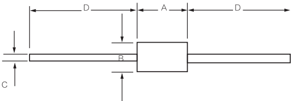
DO-15
