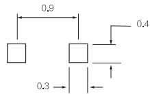
Mounting Pad Layout(mm)
