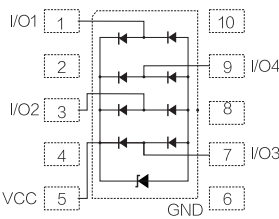
DFN- 10- 2.5X2.5X0.6- 0.5(Top view)
