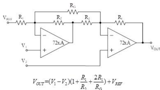
Fig. 17 Instrumentation Amplifier
