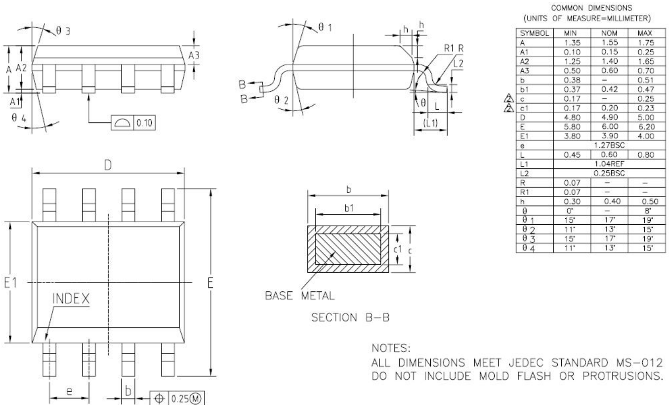
Figure 6. 8-Lead Small Outline Package [SOP]
