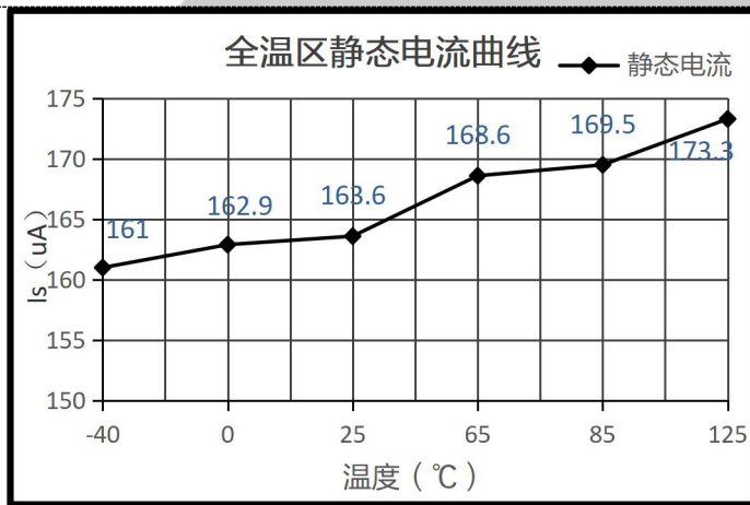
Figure 2. I S Curve In -40 °C ~ 125 °C
