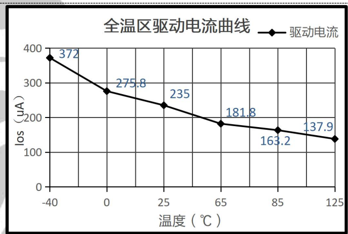
Figure 3. I OS Curve In -40 °C ~ 125 °C
