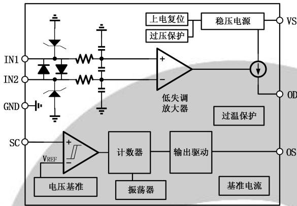
Figure 5. SS54123 G3 Block Diagram
