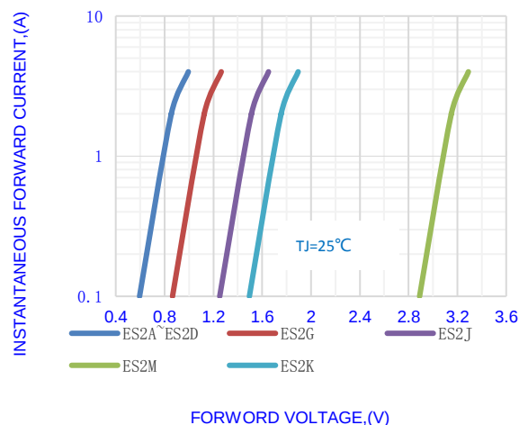
Fig.2-TYPICAL INSTANTANEOUS FORWARD
