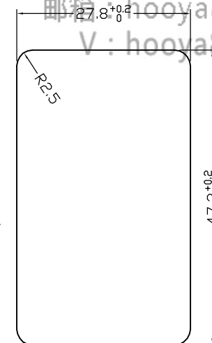
PANEL CUT-OUT
