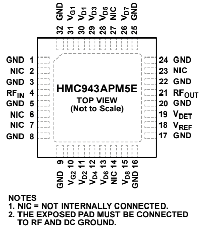
Figure 2. Pin Configuration
