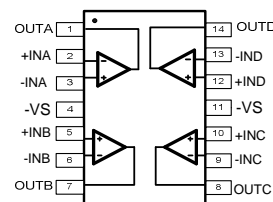
AD8634 SOP-14
