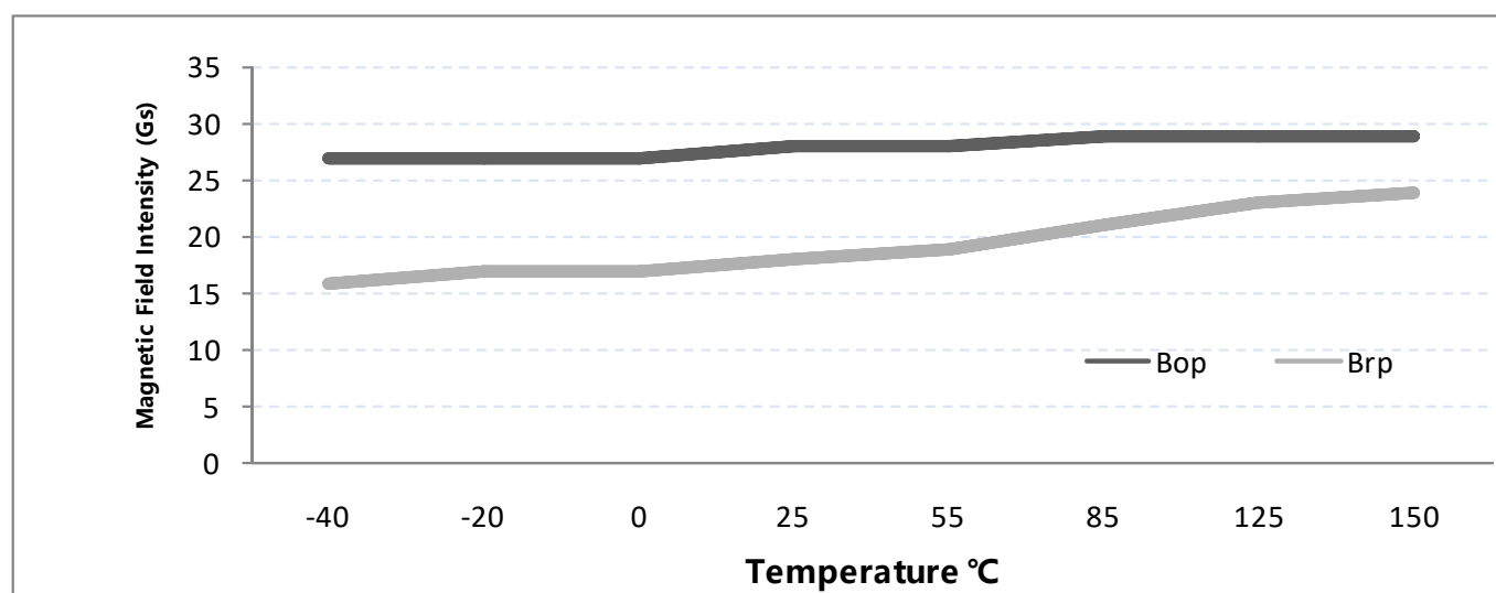
Figure.7 Magnetic Characteristics vs. Temperature (BOP & BRP)
