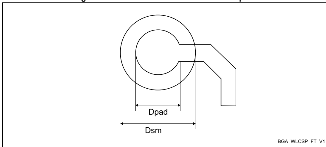
Figure 47. UFBGA100 - Recommended footprint
