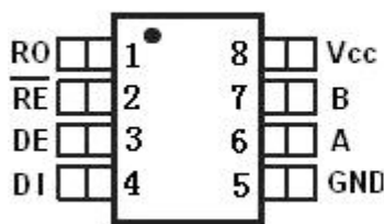
GM3085E Pin figure
