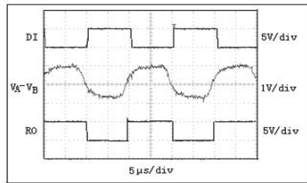
Figure 9. GM3085E System Differential Voltage at 50kHz Driving 4000ft of Cable
