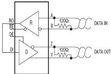
Figure 8. Line Repeater for GM3085E
