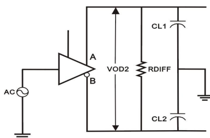
Figure3. Driver Timing Test Load
