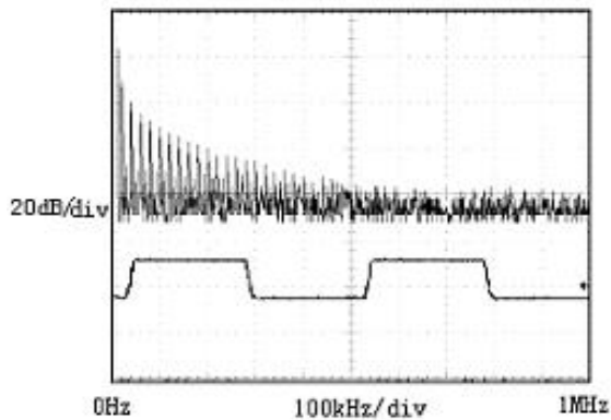
Figure 7. Driver Output Waveform and FFT Plot of GM3085E Transmitting a 20kHz Signal
