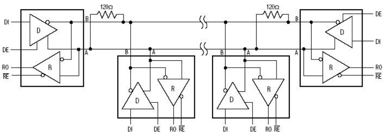
Figure 10. GM3085E Pin Configuration and Typical Half-Duplex Operating Circuit
