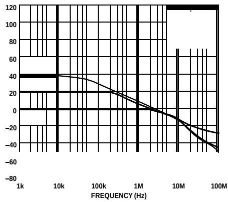
Figure 13. Closed-LoHT Gain vs. Frequency
