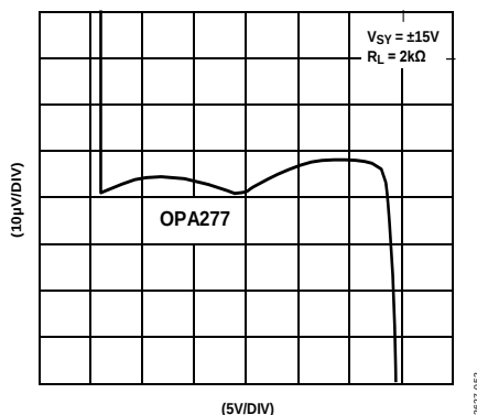
Figure 52. Gain Linearity
