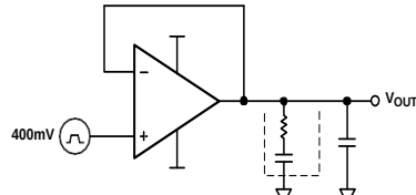
Figure 58. Snubber Network Configuration
