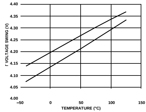
Figure 46. Output Voltage Swing vs. Temperature
