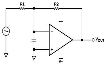
Figure 59. Stray Input Capacitance
