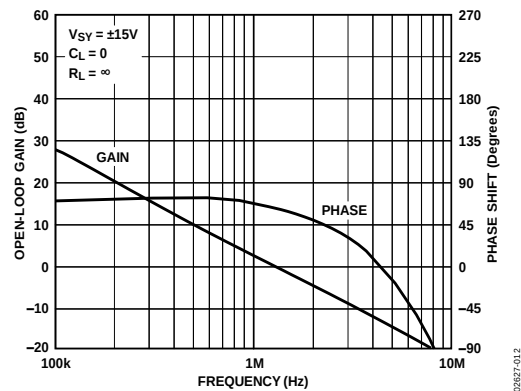
Figure 12. HTen-LoHT Gain and Phase Shift vs. Frequency
