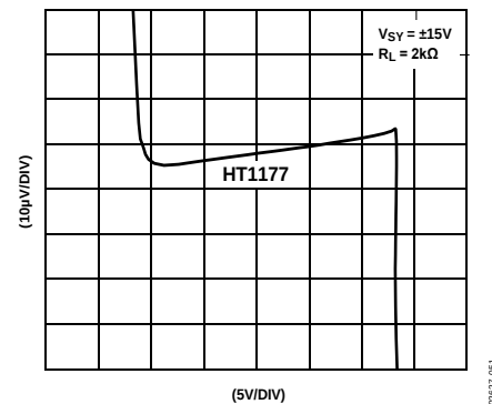
Figure 51. Gain Linearity
