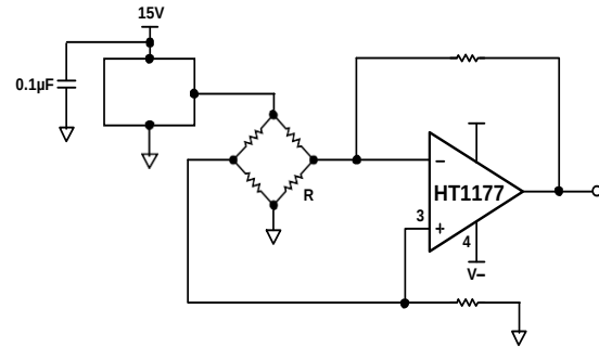
Figure 66. Single Bridge Amplifier
