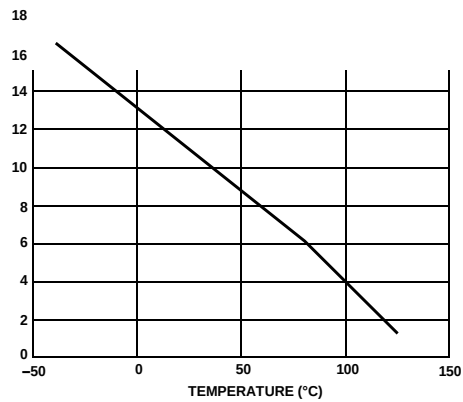
Figure 27. Input Offset Voltage vs. Temperature
