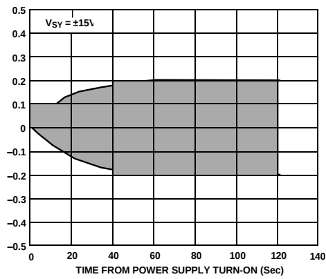
Figure 26. Warm-Up Drift
