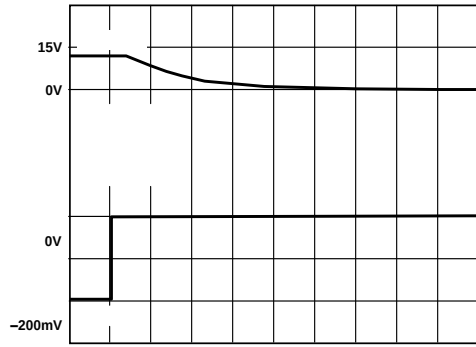
TIME (4μs/DIV) Figure 19. Negative Overvoltage Recovery
