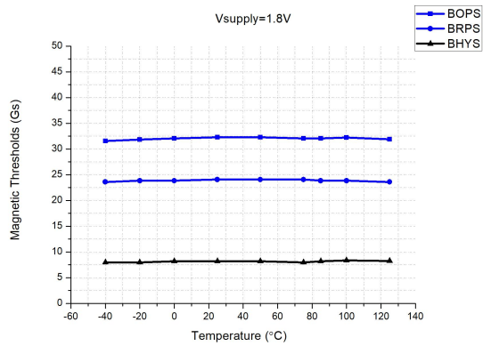
Magnetic Thresholds vs T A @VDD=1.8V
