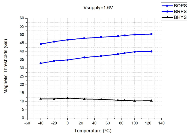
Magnetic Thresholds vs T_A @VDD=1.6V
