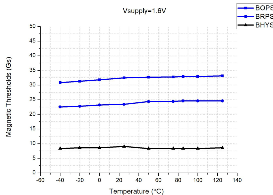
Magnetic Thresholds vs T_A @VDD=1.6V
