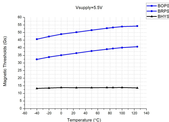
Magnetic Thresholds vs T_A @VDD=5.5V
