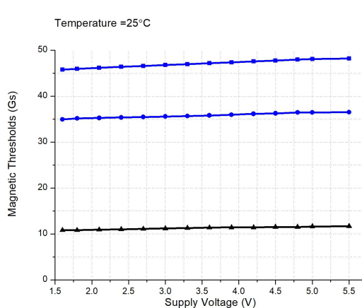
Magnetic Thresholds vs. Supply Voltage @ T_A=25^{\circ}C
