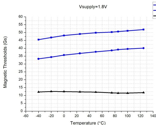
Magnetic Thresholds vs T_A @VDD=1.8V
