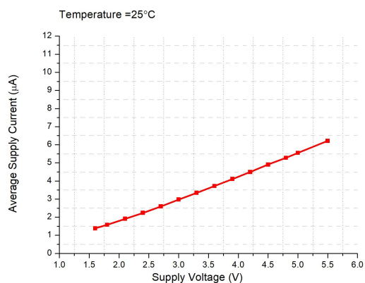
Current Consumption vs. Supply Voltage @ T_A=25^\circ\text{C}
