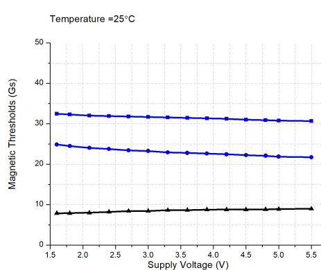
Magnetic Thresholds vs. Supply Voltage @ T_A=25^{\circ}C
