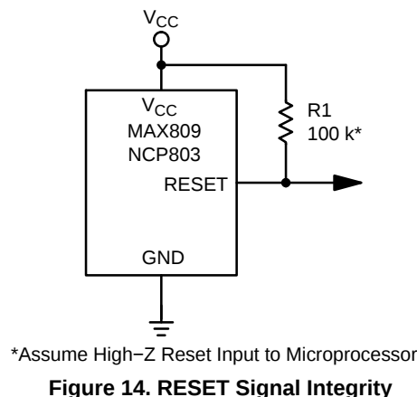
Figure 14. RESET Signal Integrity
