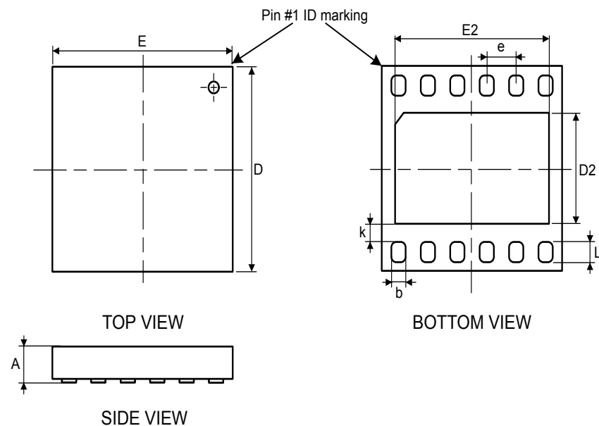
Figure 83. UFDFPN12 - Outline
