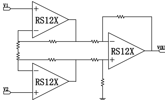
Figure2. Amplifier instrumentation amplifier
