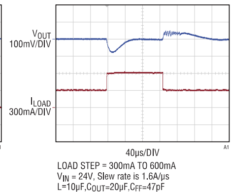
Load Transient, V OUT = 5V
