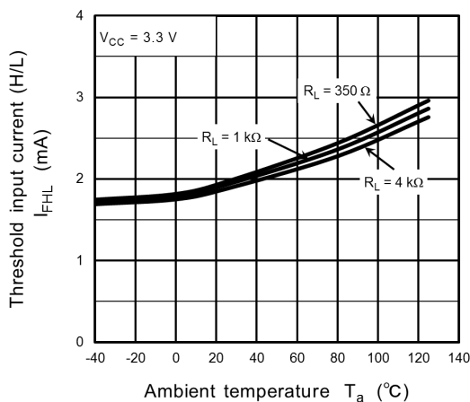
Fig. 13.2.8 I_{FHL} - T_a
