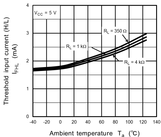
Fig. 13.2.7 I_{FHL} - T_a
