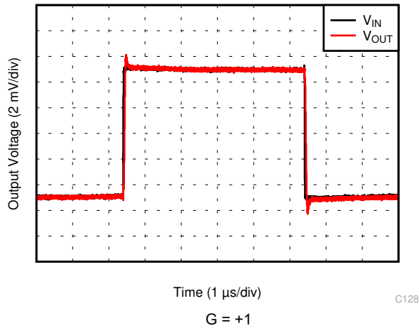
图 6-27. Small-Signal Step Response
