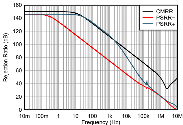
图 6-13. PSRR and CMRR vs Frequency
