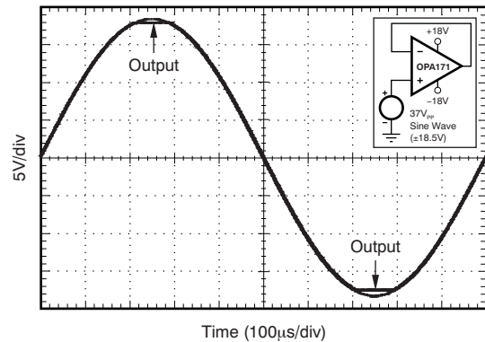
Figure 37. 无相位反转
