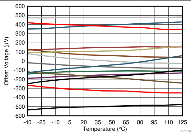
图 7-3. Offset Voltage vs Temperature
