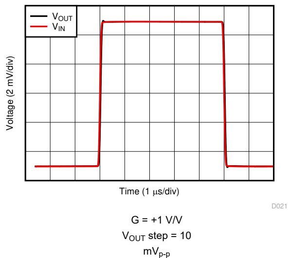
图 7-23. Small-Signal Step Response
