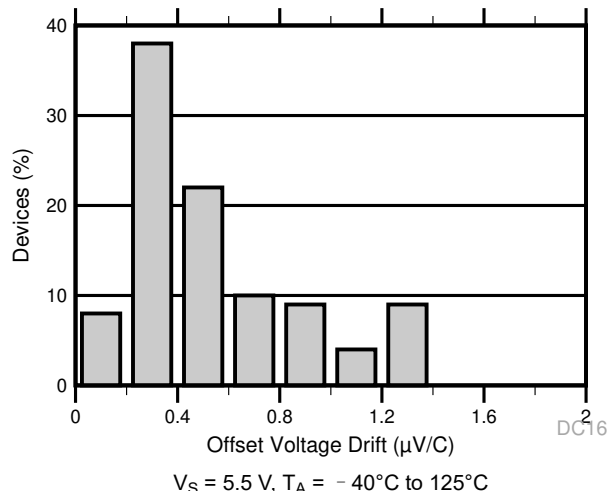
图 7-2. Offset Voltage Drift Distribution
