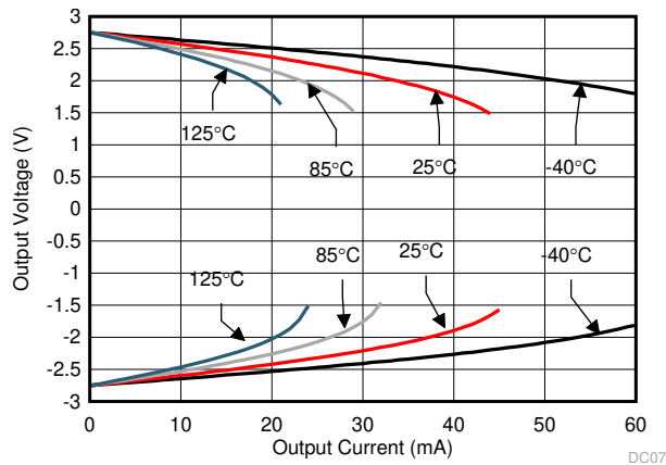
图 7-31. Output Voltage Swing vs Output Current
