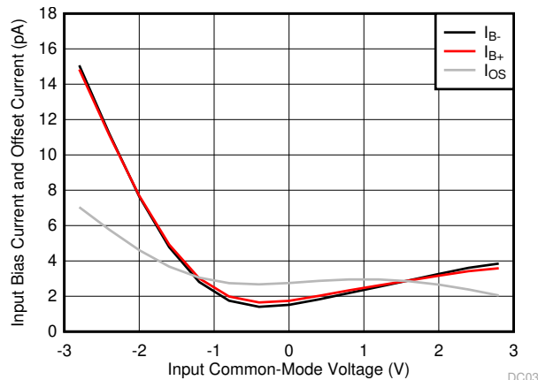
图 7-7. Input Bias Current and Offset Current vs Common-Mode Voltage
