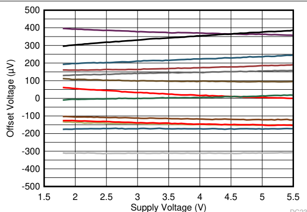
图 7-5. Offset Voltage vs Power Supply
