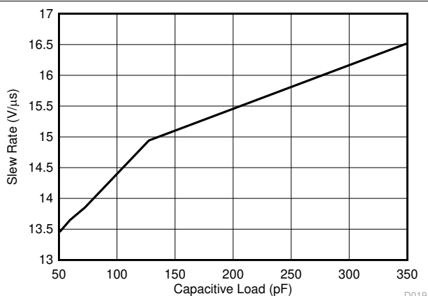
图 7-21. Slew Rate vs Capacitive Load
