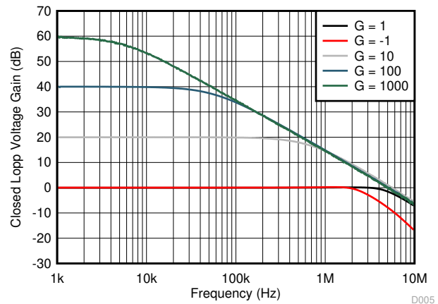
图 7-16. Closed Loop Voltage Gain vs Frequency
