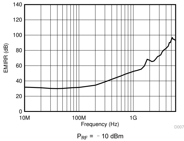
图 7-37. Electromagnetic Interference Rejection Ratio Referred to Noninverting Input (EMIRR+) vs Frequency
