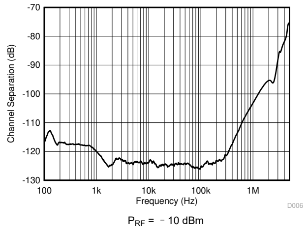
图 7-38. Channel Separation vs Frequency
