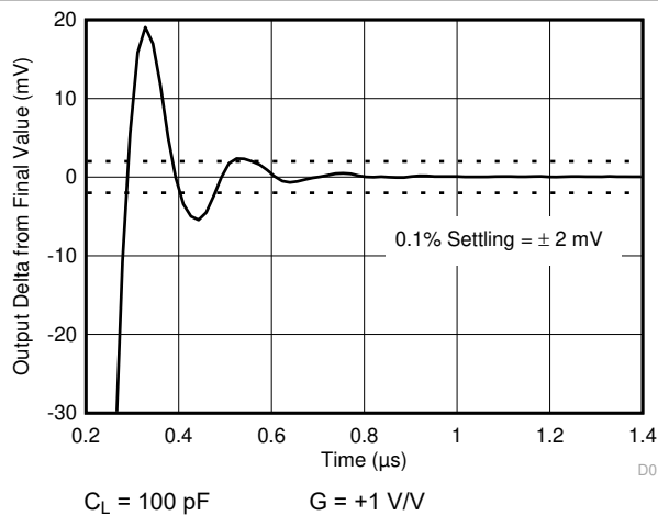
图 7-27. Positive Large-Signal Settling Time
