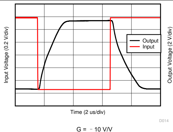
图 7-22. Overload Recovery
