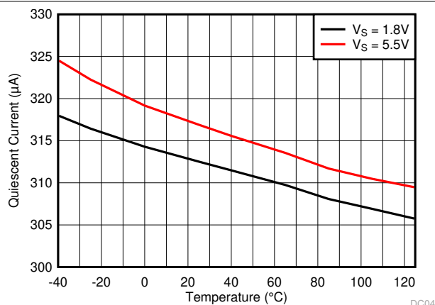
图 7-35. Quiescent Current vs Temperature
