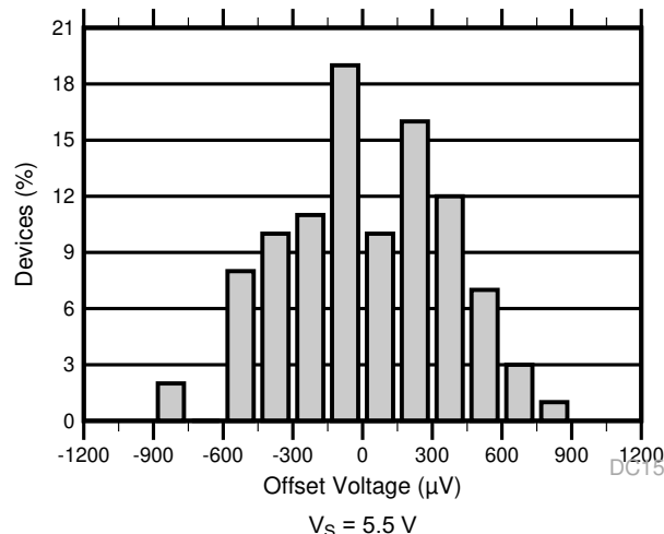
图 7-1. Offset Voltage Production Distribution
