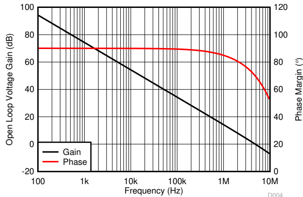
图 7-13. Open Loop Voltage Gain and Phase vs Frequency
