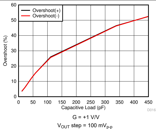
图 7-19. Small-Signal Overshoot vs Load Capacitance
