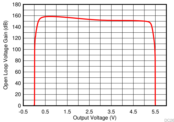
图 7-15. Open Loop Voltage Gain vs Output Voltage
