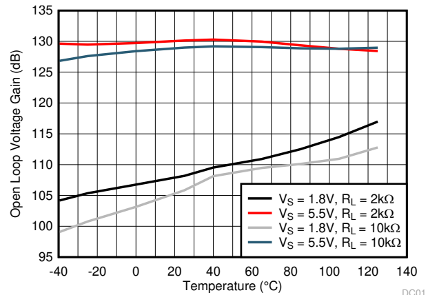
图 7-14. Open Loop Voltage Gain vs Temperature
