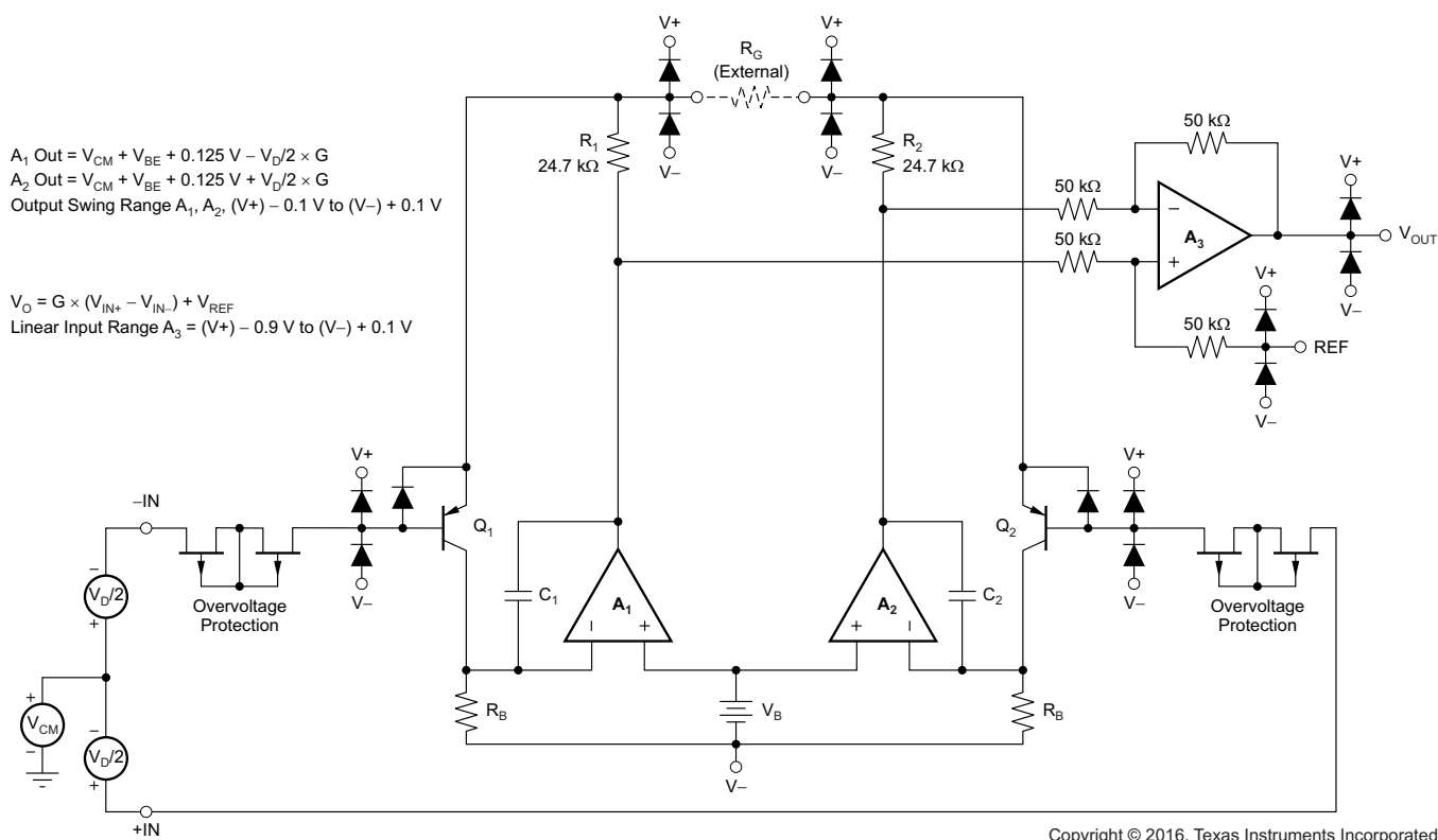
图 65. INA826S Simplified Circuit Diagram
