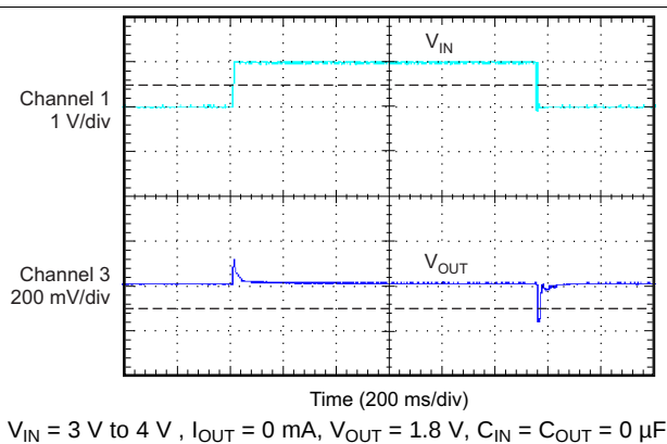
Figure 12. Line Transient
