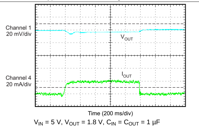
Figure 14. 0-mA to 20-mA Load Transient
