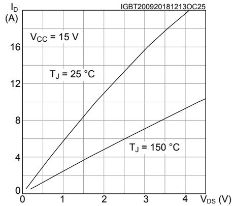
Figure 11. Output characteristics
