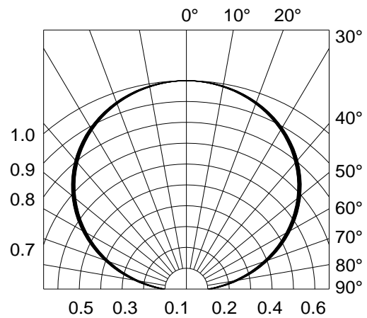
Fig.6-Radiation Diagram Ta=25°C
