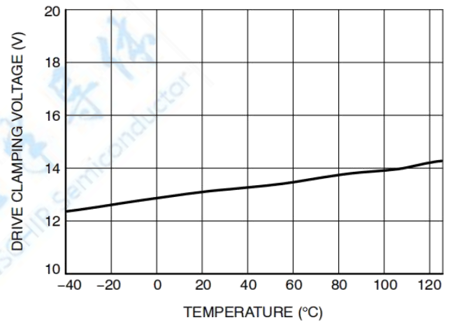
Figure 20. Drive Clamping Voltage vs. Junction Temperature
