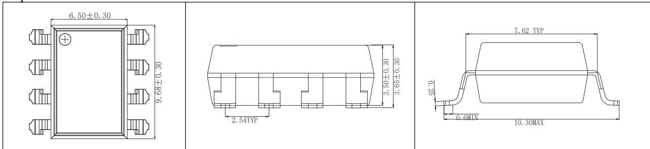
8pin SMD
