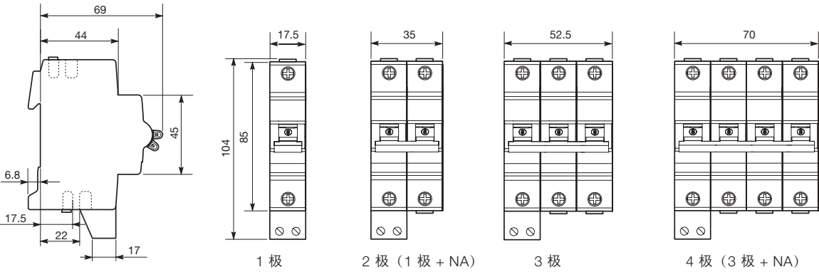
S200/M/P/MDC (带底部安装的辅助触头)
