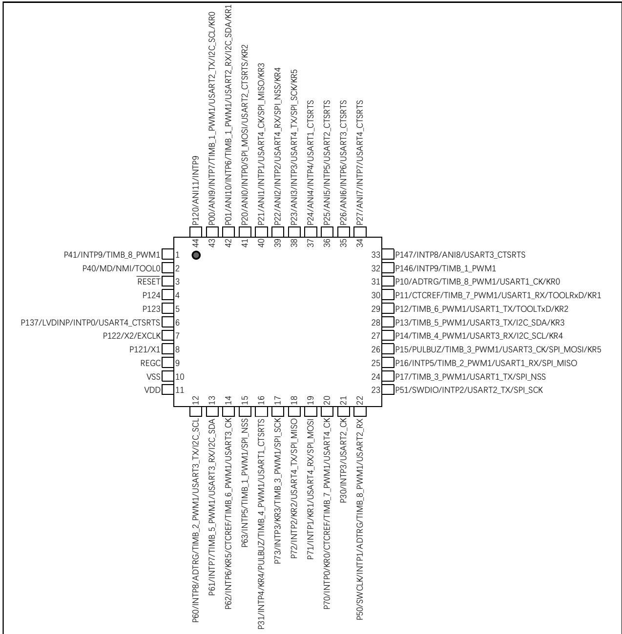
LQFP44
