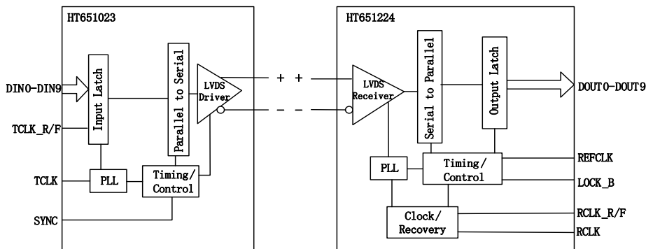
Figure 1. Functional Description
